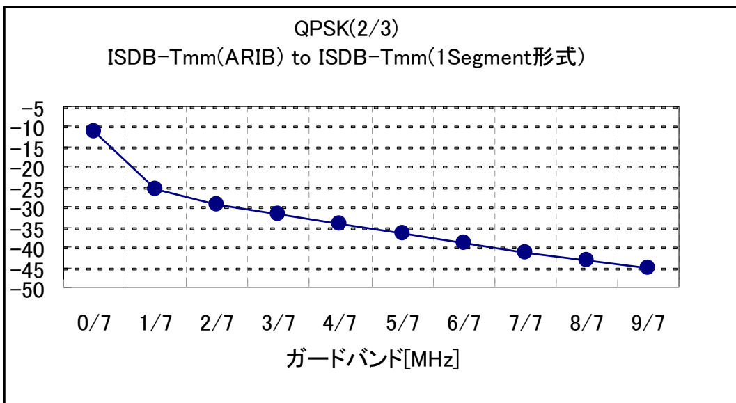
(b) QPSK (2/3)
