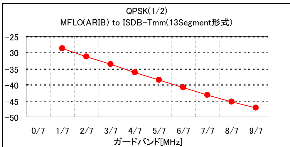
(c) QPSK (1/2)
