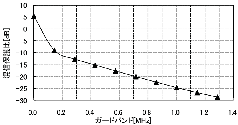
(b) QPSK (2/3)
