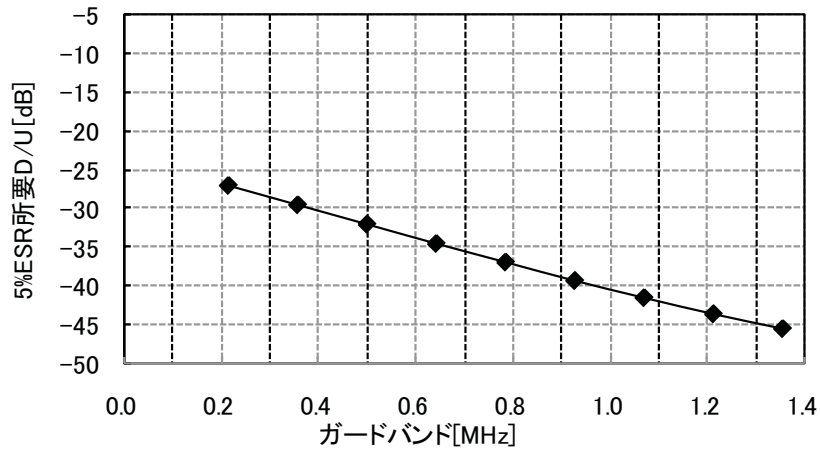
(b) QPSK (2/3)
