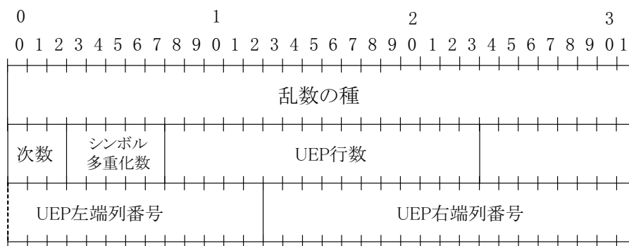
図3.1.5.4-24 FEC-OTI-Scheme-Specific-Info (UEP対応)
