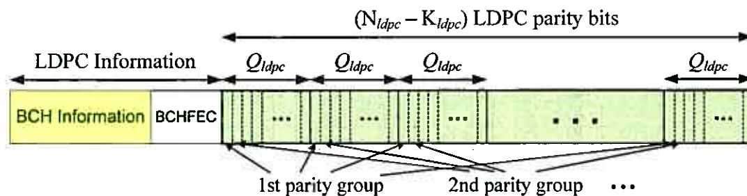
Figure 26: Parity bit groups in an FEC block
