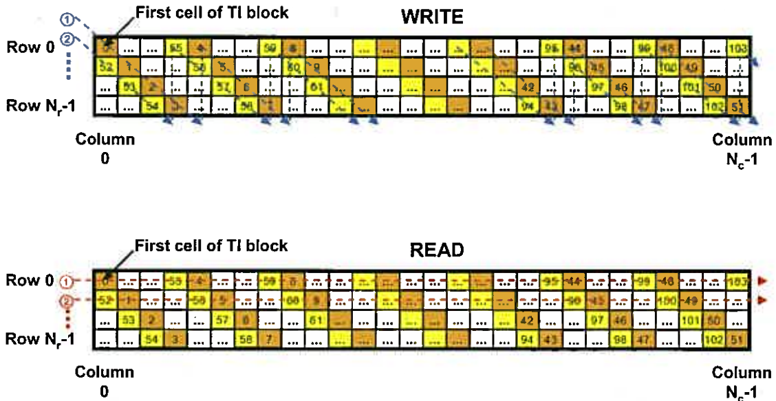
Figure 29: Time interleaving of L1 data ( N_{MOD\_TOTAL}=208 , N_{LI\_TI\_DEPTH}=4 )
