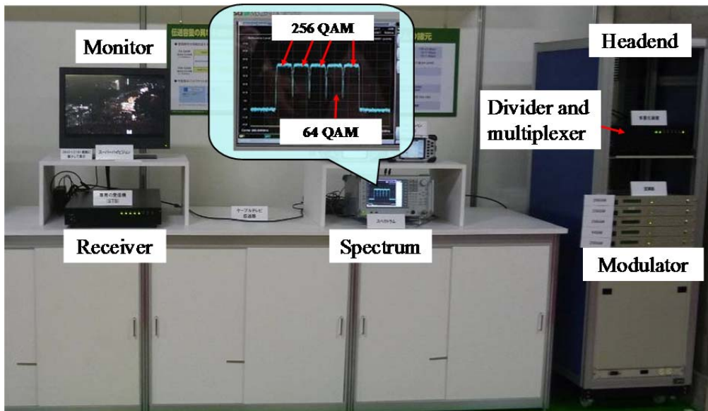
Fig. 7 Setup for UHDTV transmission.
