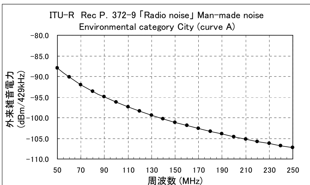
図4-1 外来雑音電力 (ITU-R Rec P. 372-9 「Radio noise」 Man-made noise Environmental category City (curve A))
