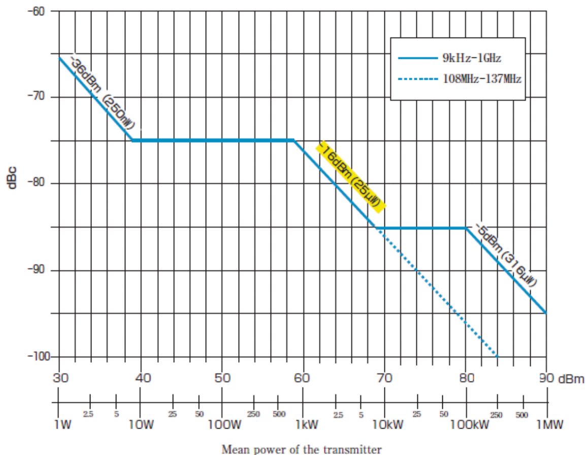
Figure 4.1 : Spurious emission limits for FM sound broadcasting transmitters
