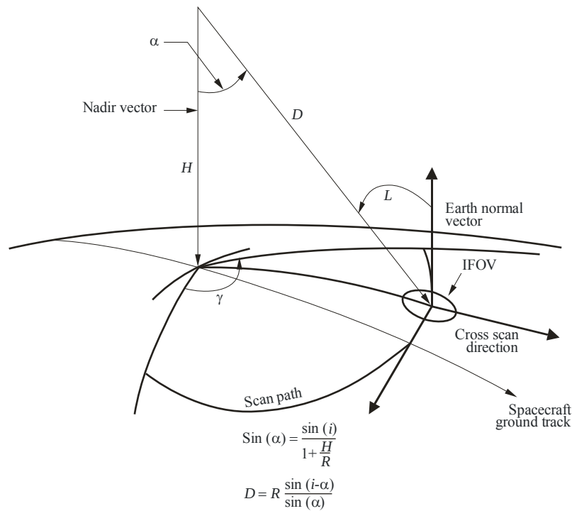
FIGURE 6 Scanning configuration
