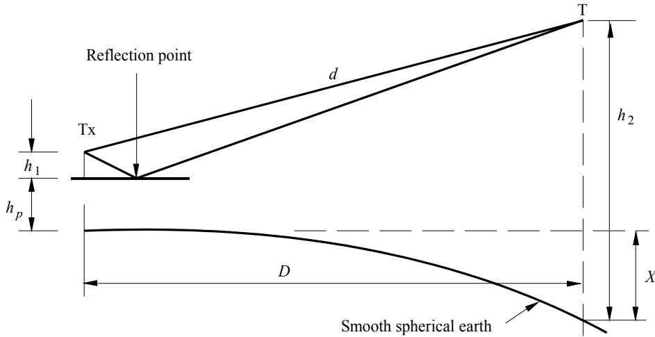
FIGURE 8 Two-ray geometry
