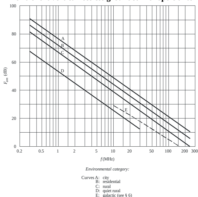
FIGURE 10 Median values of man-made noise power for a short vertical lossless grounded monopole antenna
