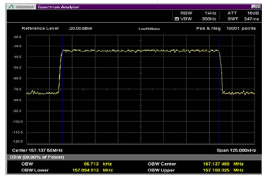
32X16QAM
