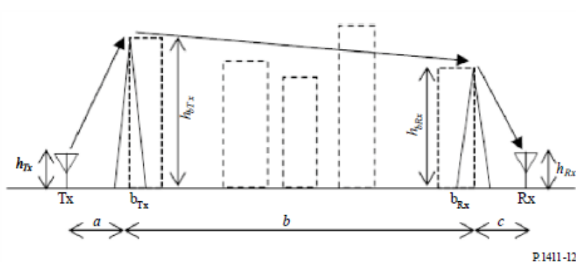
Side view of building geometry and parameters
