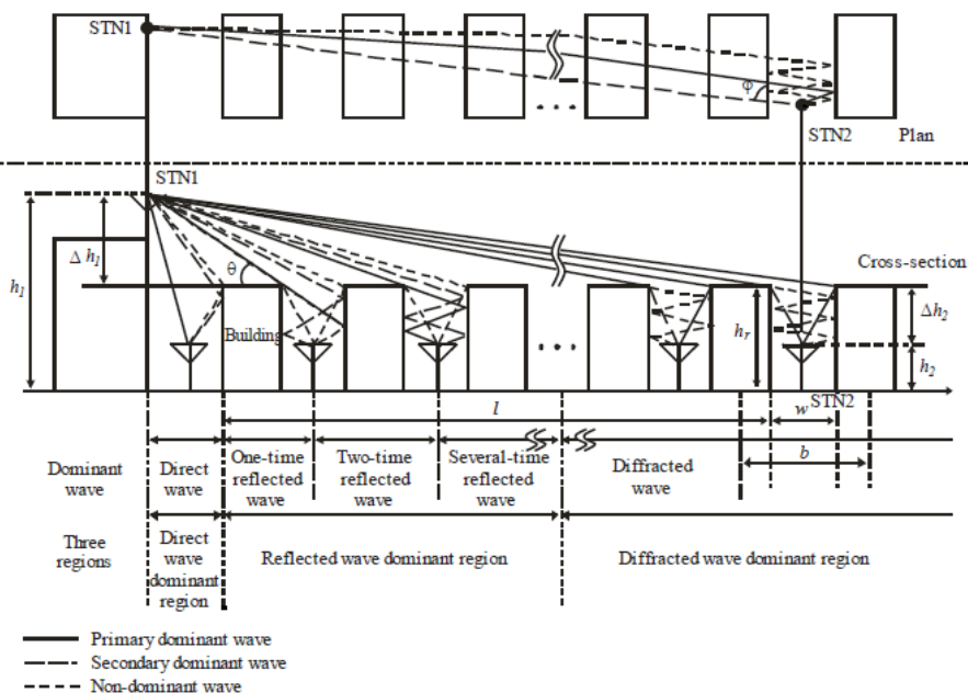
FIGURE 2 Definition of parameters for the NLoS1 case
