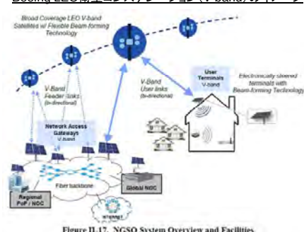
Figure 11-17. NGSO System Overview and Facilities
