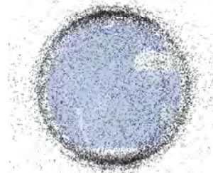
Space Debris (Nasa earth observatory)
