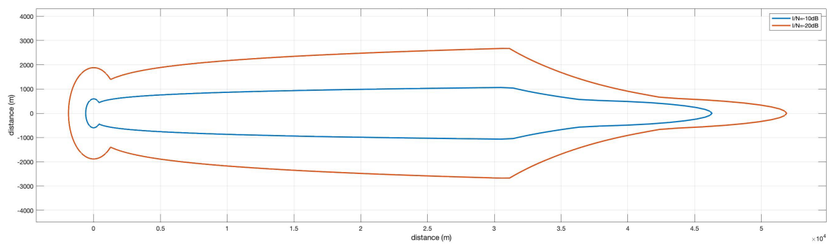
参考図 6.3-11 Pattern2-2 (Rec. ITU-R F.1245, VLP, 25mW, Outdoor, Body Loss なし)
