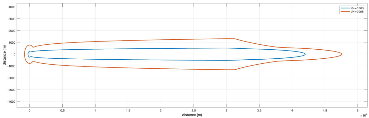
参考図 6.3-10 Pattern1-2 (Rec. ITU-R F.1245, LPI, 200mW, Indoor)
