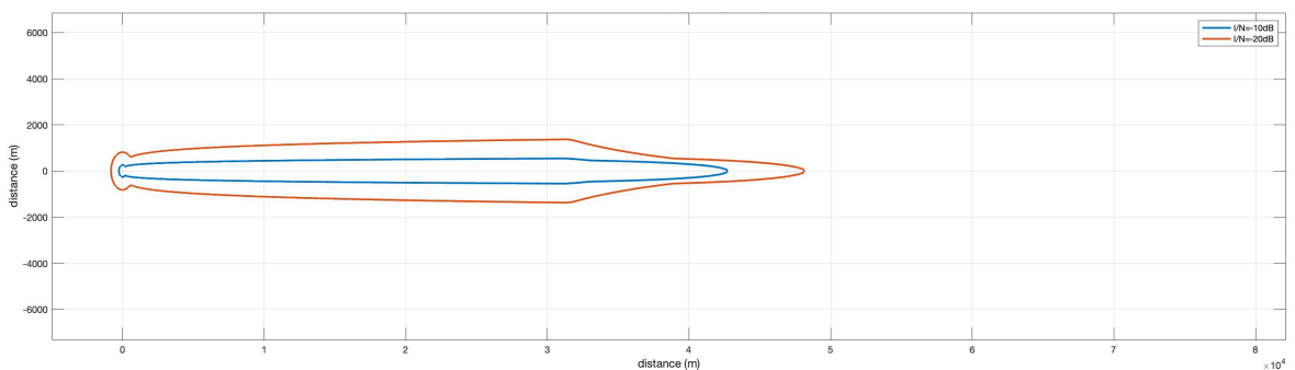
参考図 6.3-31 Pattern1-2 (Rec. ITU-R F.1245, LPI, 200mW, Indoor)
