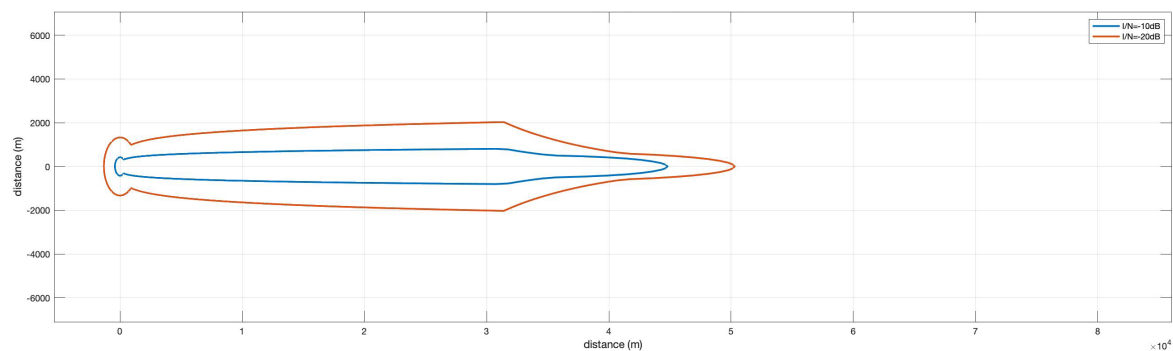
参考図 6.3-24 Pattern3-2 (Rec. ITU-R F.1245, VLP, 25mW, Outdoor, Body Loss あり)
