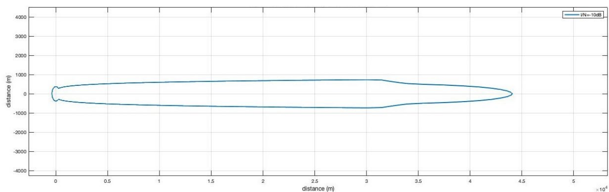
図 6.3-12 Pattern3-2 (Rec. ITU-R F.1245, VLP, 25mW, Outdoor, Body Loss あり)
