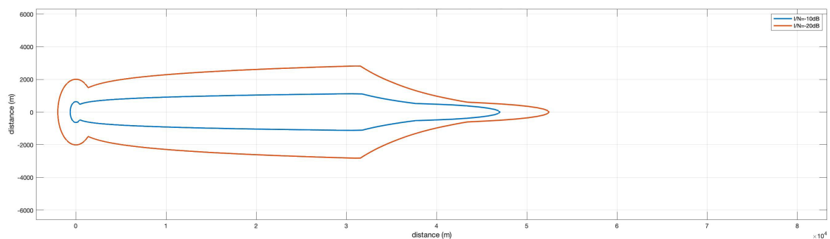
参考図 6.3-32 Pattern2-2 (Rec. ITU-R F.1245, VLP, 25mW, Outdoor, Body Loss なし)
