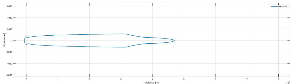
図 6.3-23 Pattern2-2 (Rec. ITU-R F.1245, VLP, 25mW, Outdoor, Body Loss なし)
