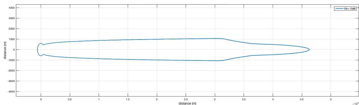
図 6.3-11 Pattern2-2 (Rec. ITU-R F.1245, VLP, 25mW, Outdoor, Body Loss なし)
