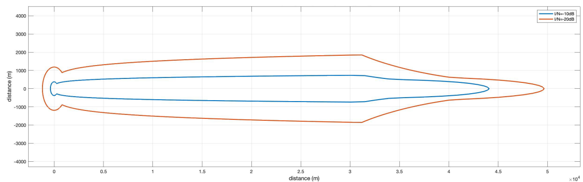
参考図 6.3-12 Pattern3-2 (Rec. ITU-R F.1245, VLP, 25mW, Outdoor, Body Loss あり)
