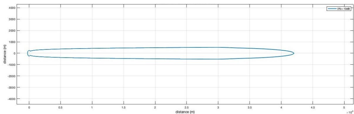
図 6.3-10 Pattern1-2 (Rec. ITU-R F.1245, LPI, 200mW, Indoor)
