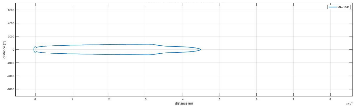
図 6.3-24 Pattern3-2 (Rec. ITU-R F.1245, VLP, 25mW, Outdoor, Body Loss あり)
