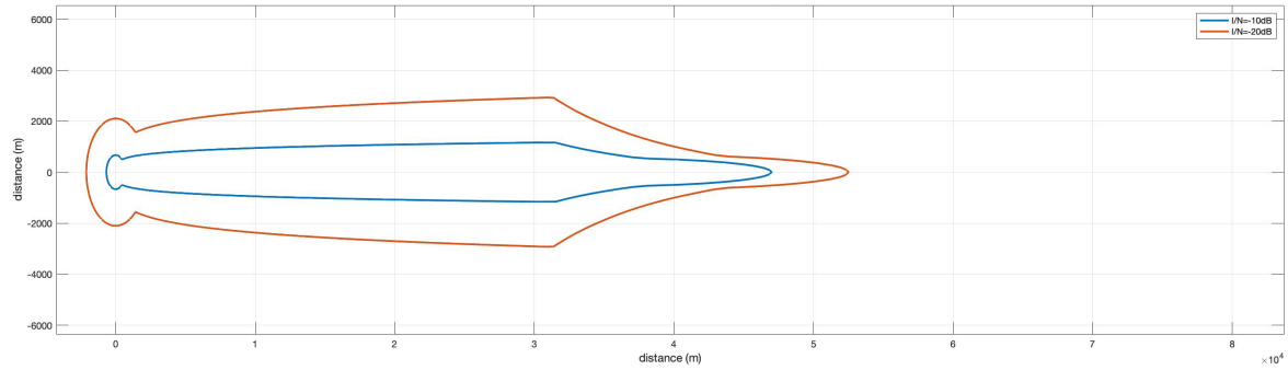
参考図 6.3-23 Pattern2-2 (ITU-R F.1245, VLP, 25mW, Outdoor, Body Loss なし)
