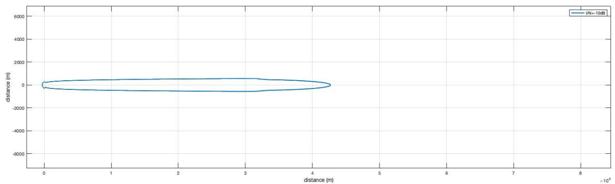
図 6.3-22 Pattern1-2 (ITU-R F.1245, LPI, 200mW, Indoor)
