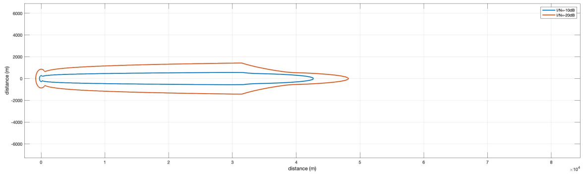
参考図 6.3-22 Pattern1-2 (ITU-R F.1245, LPI, 200mW, Indoor)
