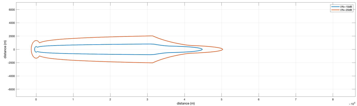
参考図 6.3-24 Pattern3-2 (ITU-R F.1245, VLP, 25mW, Outdoor, Body Loss あり)
