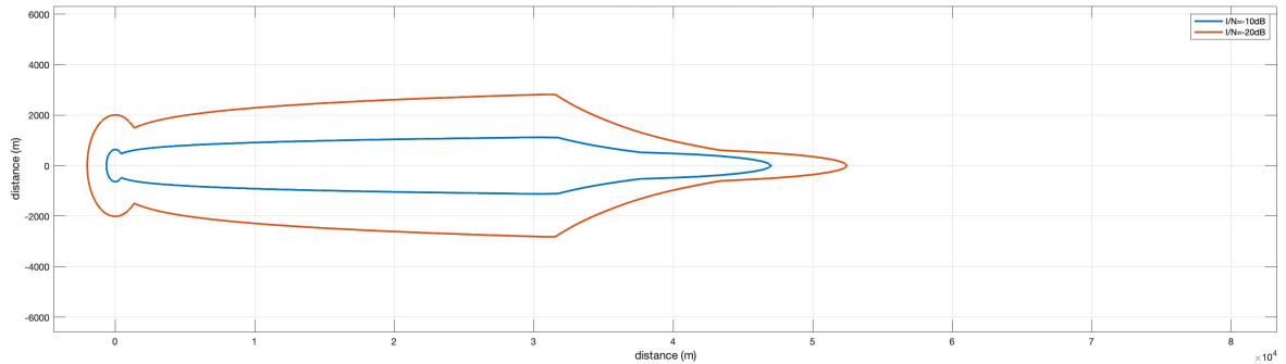
参考図 6.3-32 Pattern2-2 (ITU-R F.1245, VLP, 25mW, Outdoor, Body Loss なし)
