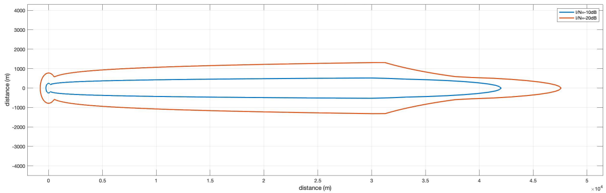
参考図 6.3-10 Pattern1-2 (ITU-R F.1245, LPI, 200mW, Indoor)
