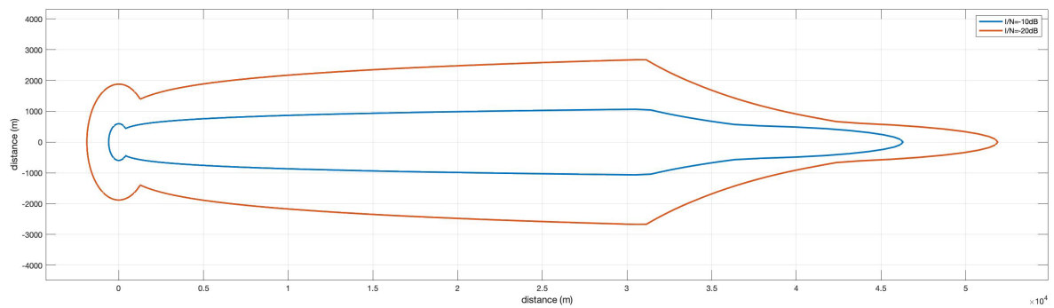
参考図 6.3-11 Pattern2-2 (ITU-R F.1245, VLP, 25mW, Outdoor, Body Loss なし)
