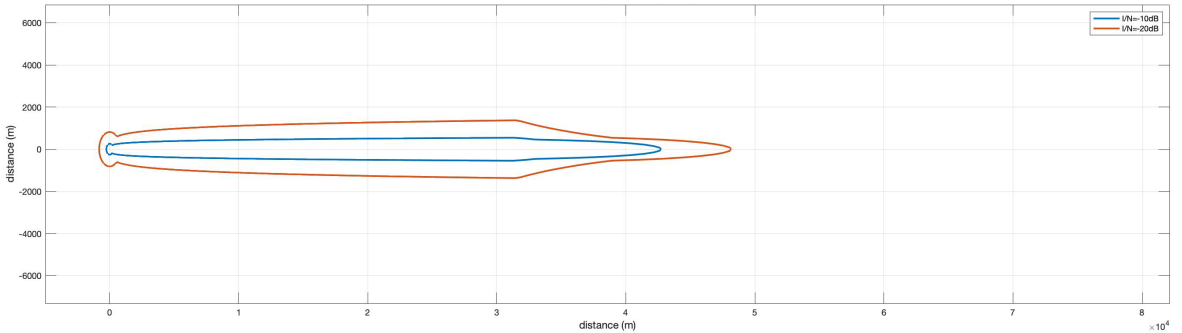
参考図 6.3-31 Pattern1-2 (ITU-R F.1245, LPI, 200mW, Indoor)
