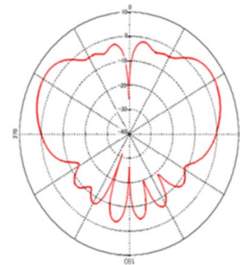
ITS車載(垂直面)
