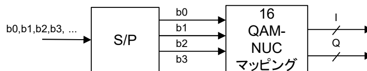
(c) 16 QAM-NUC
