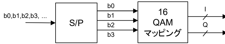
(b) 16QAM
