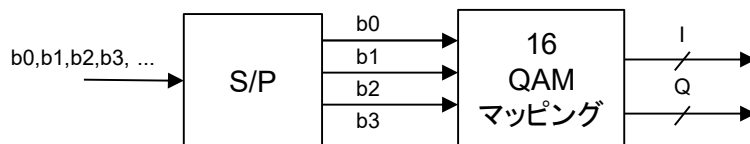
(b) 16 QAM
