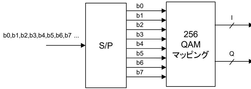
(f) 256 QAM
