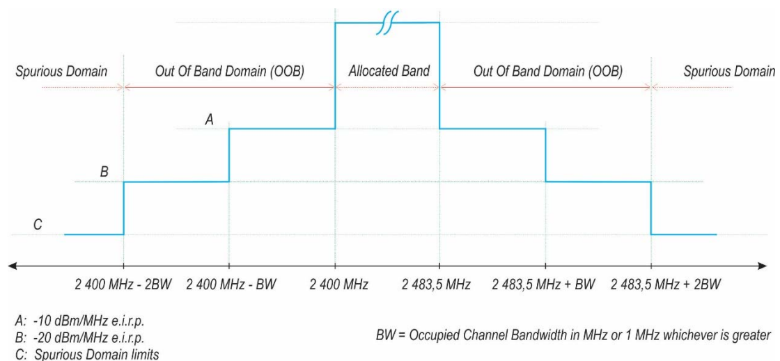
Figure 1: Transmit mask
