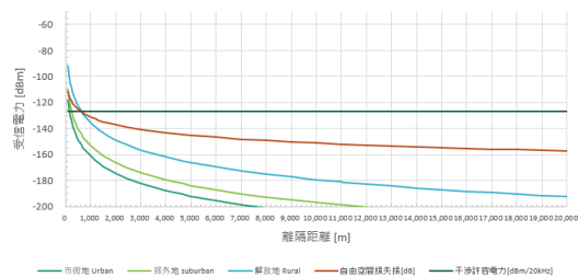
参図2-21 RKE 帯域外 -36.02dBm/100kHz (-43.01dBm/20kHz)
