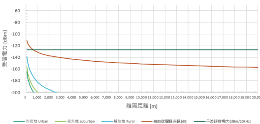
参図2-24 RKE 帯域外 -36.02dBm/100kHz (-43.01dBm/20kHz)
