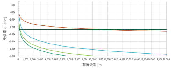
参图2-14 RKE 带域外 -36.02dBm/100kHz (-43.01dBm/20kHz)
