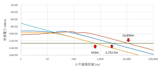
参図2-10 RKE 帯域外 -36.02dBm/100kHz (-43.01dBm/20kHz)
