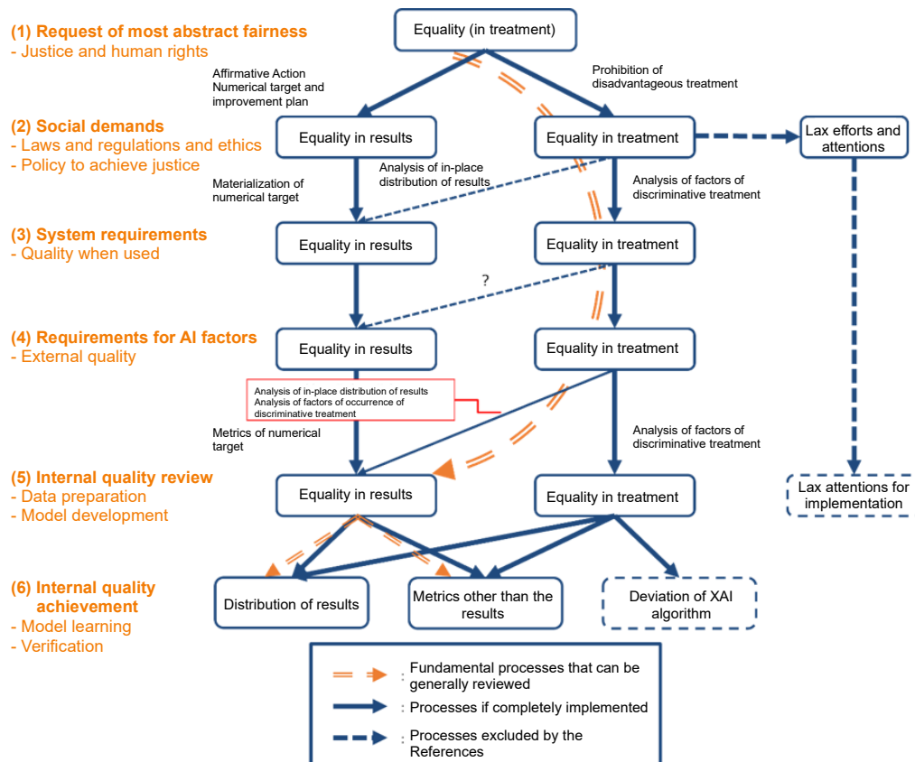
Figure 30. Illustration of a process structure to assure the fairness quality
