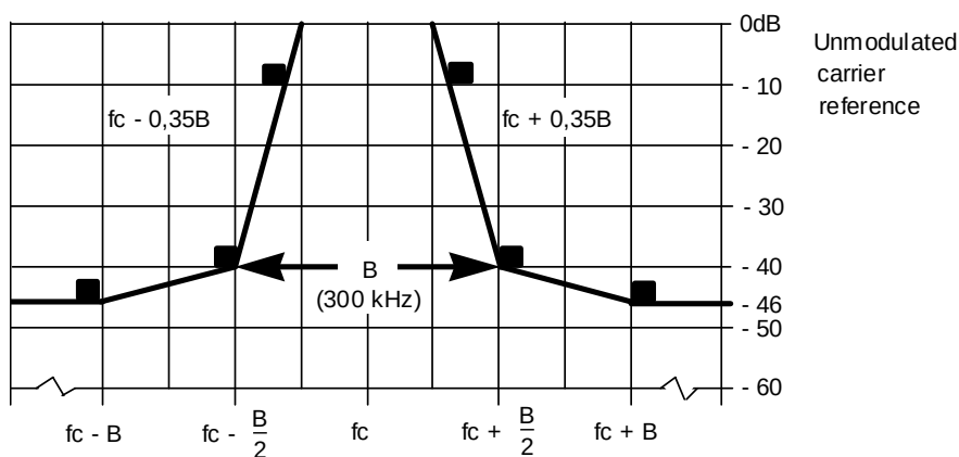
図 3 Spectral mask for analogue or digital modulation with B = 300 kHz
