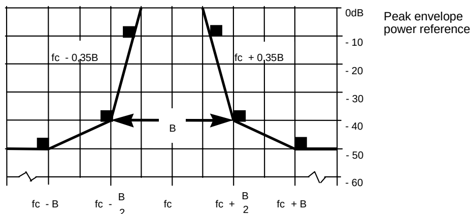
図 4 Scaleable Spectral mask for digital modulation with B = 600, 1\ 200 kHz
