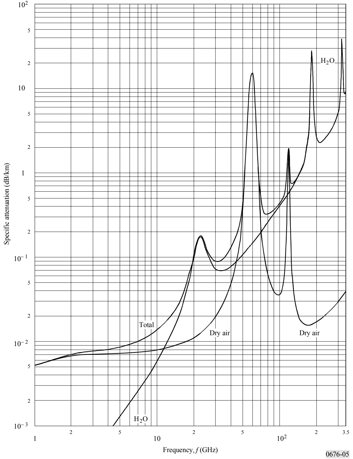
Specific attenuation due to atmospheric gases
